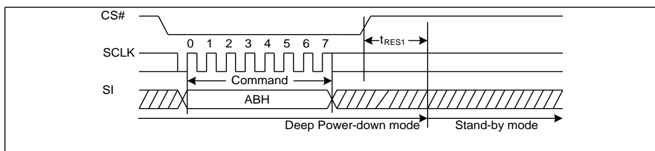
Figure23. Release Power-Down/Read Device ID Sequence Diagram
