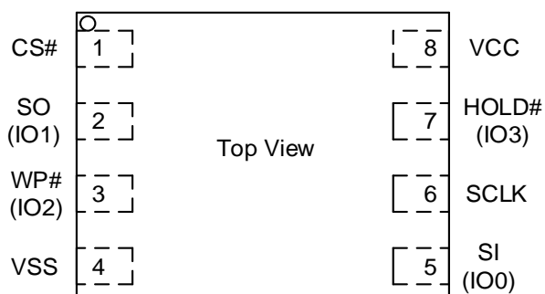
8 - LEAD WSON/USON/LGA
