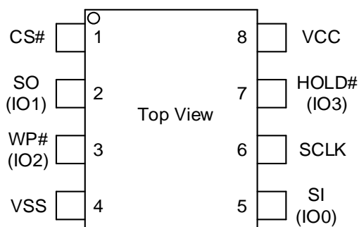
8 - LEAD VSOP/SOP
