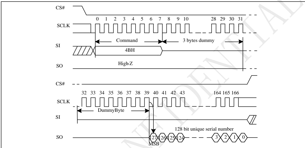
Figure 10-60Read Unique ID (RUID) Sequence (Command 4B)
