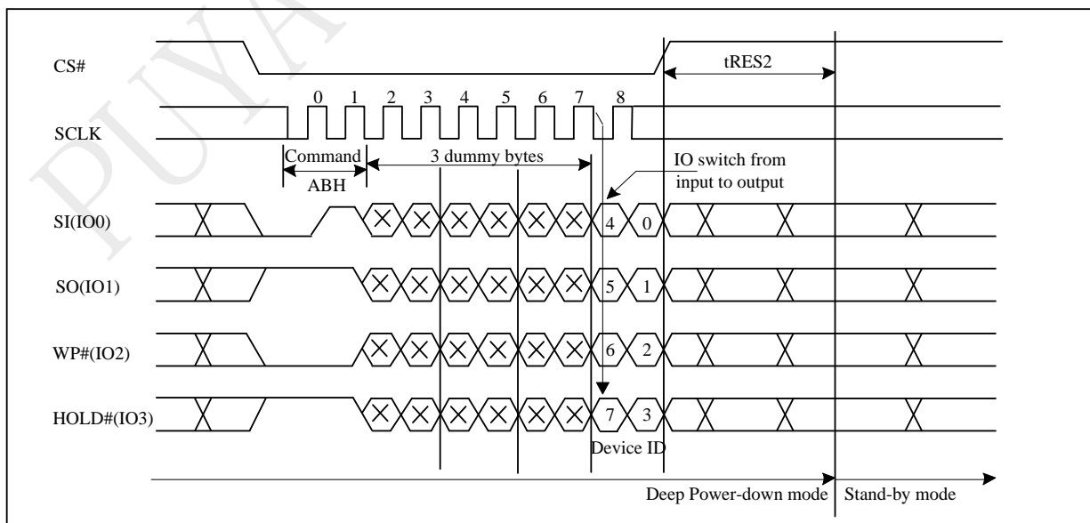
Figure 10-44a Read Electronic Signature (RES) Sequence (QPI)
