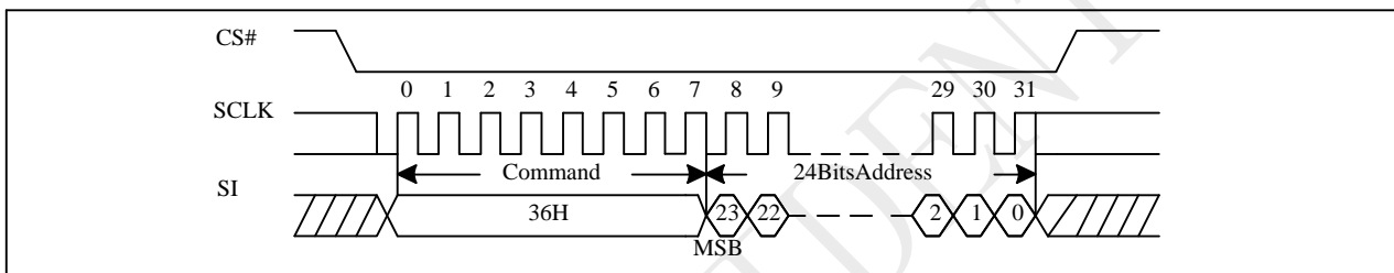
Figure 10-53 Individual Block Lock (Command 36H)
