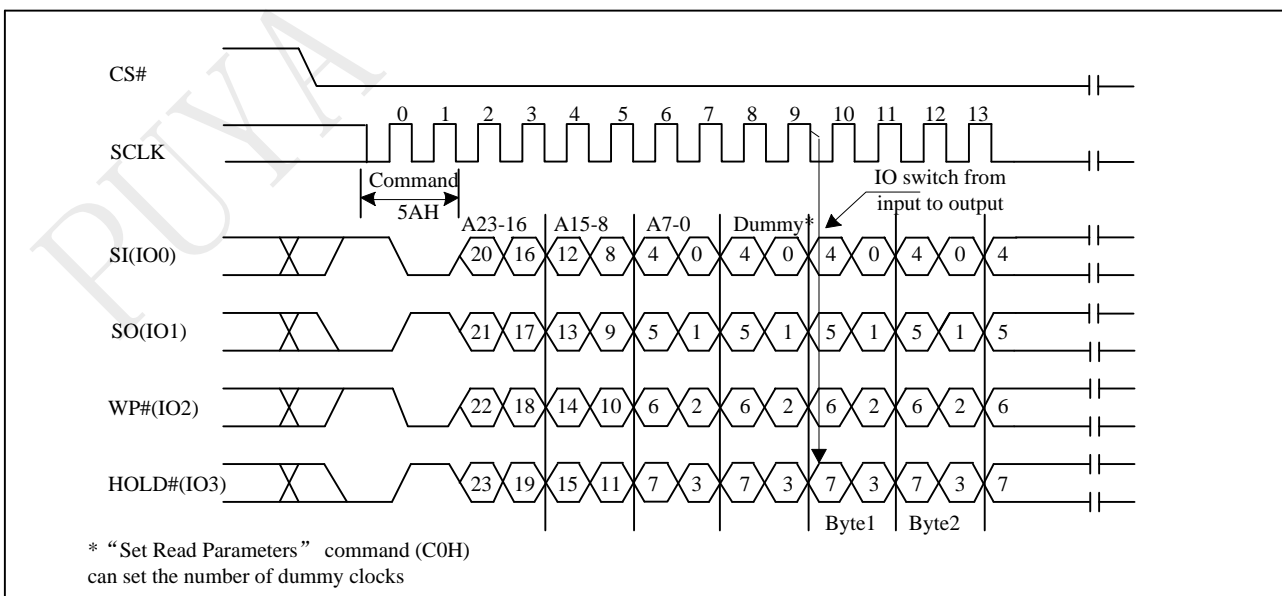
Figure 10-61a Read Serial Flash Discoverable Parameter (RDSFDP) Sequence(QPI)
