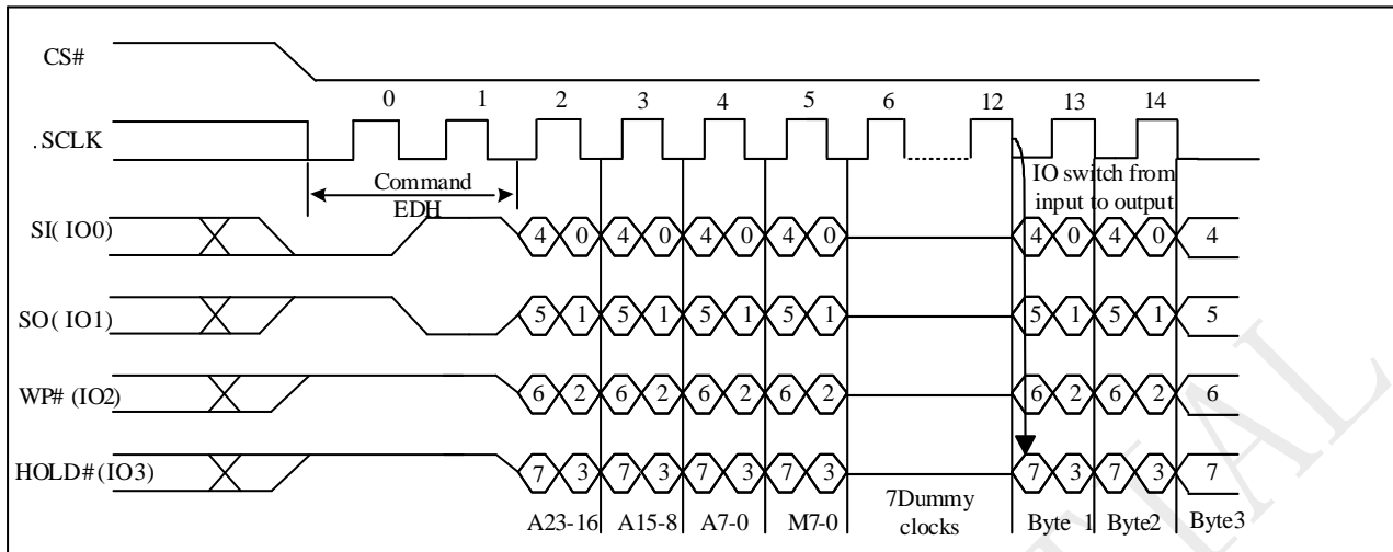
Figure 10-20bDTR 4IO Read Mode Sequence (QPI EDM5-4 ≠ (1,0))
