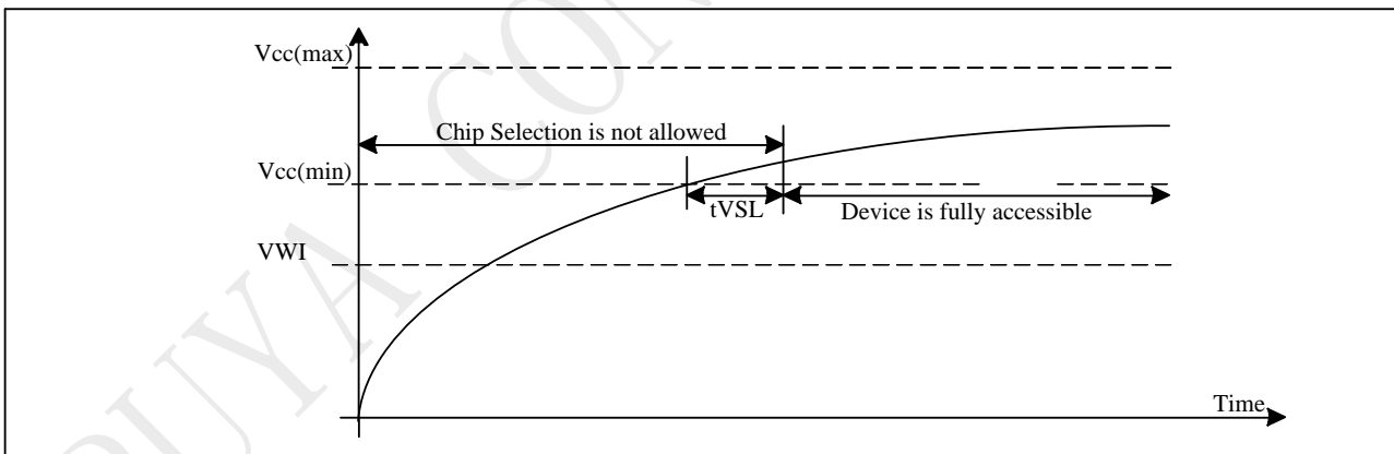
Figure 5-9 Power-up Timing
