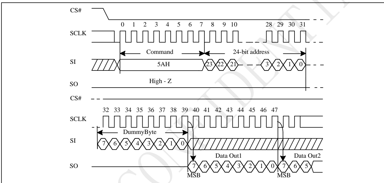
Figure 10-61 Read Serial Flash Discoverable Parameter (RDSFDP) Sequence
