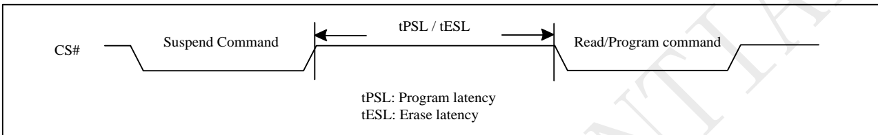
Figure 10-50a Suspend to Read/Program Latency(QPI)
