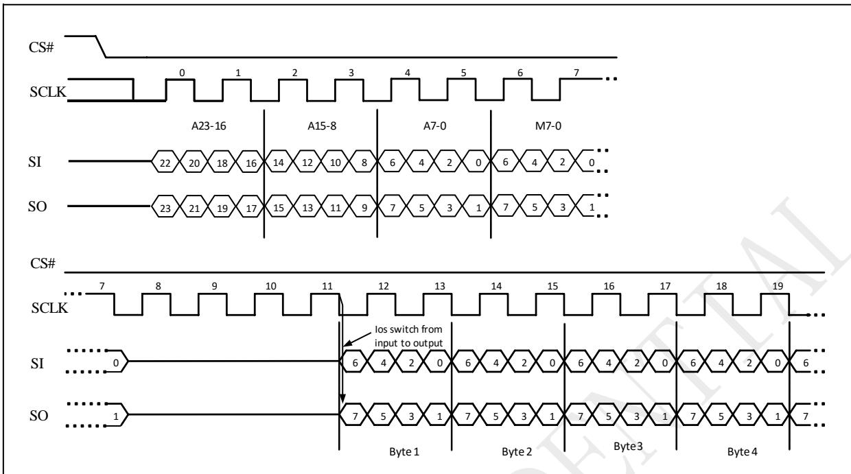
Figure 10-16aDTR 2IO Continuous Read Sequence (Command BD M5-4 = (1,0))
