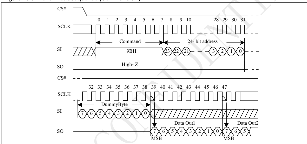
Figure 10-37 Buffer Read Sequence (Command 9B)
