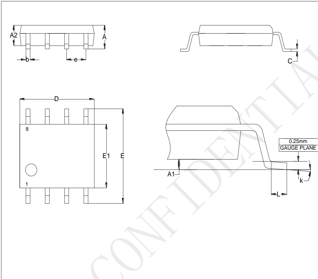
Common Dimensions (Unit of Measure=millimeters)
