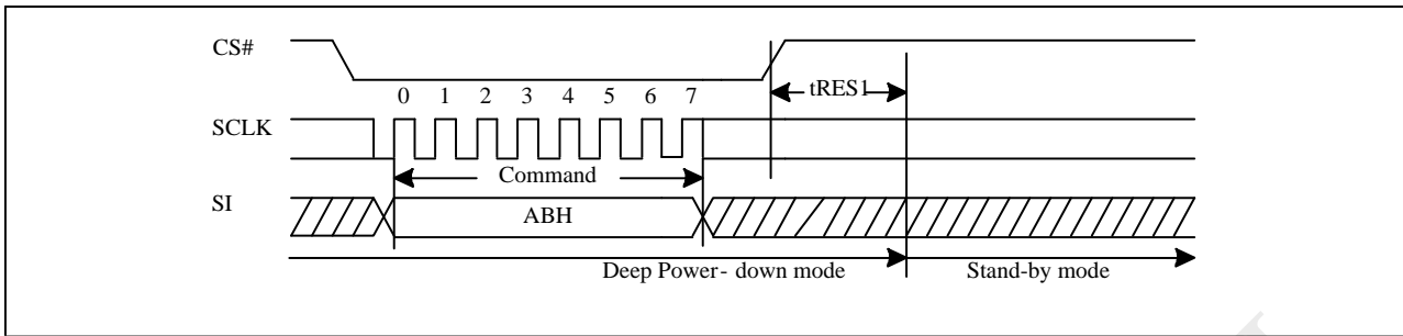
Figure 10-44b Release from Deep Power-down (RDP) Sequence (Command AB)
