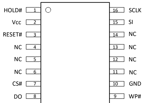
16-PinSOP (300mil)
