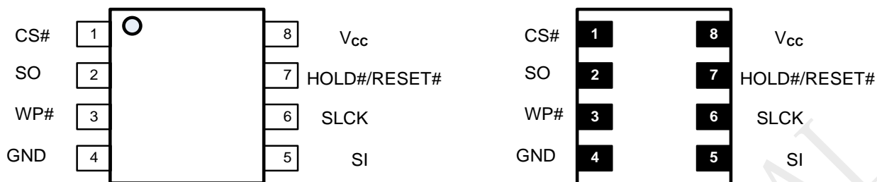
8-PIN SOP (208mil)
