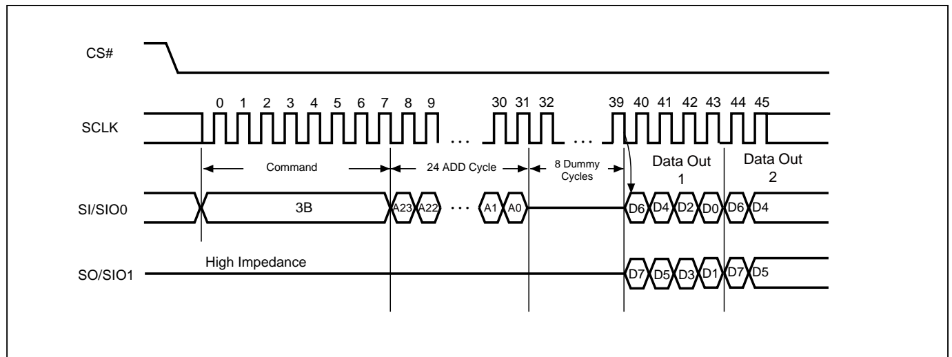
Figure 33. Dual Read Mode Sequence
