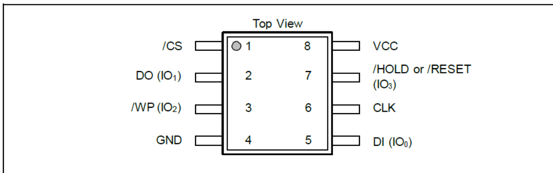
Figure 3.1 8-pin SOP 150/208mil
