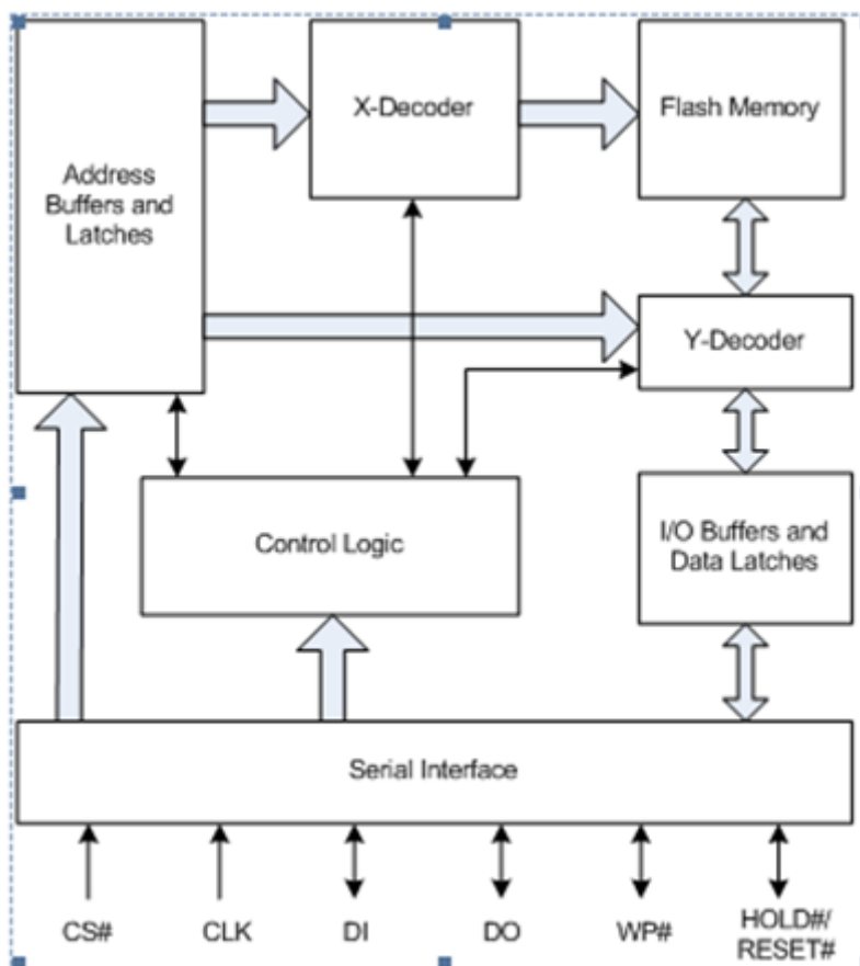
Figure 2.1 Block Diagram
